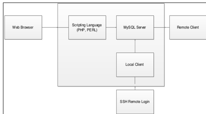
Figure 1. MySQL server prototype stage in this research.
