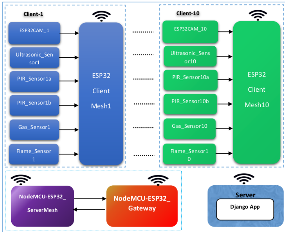
Figure 1 Block Diagram SCHMV1.0
