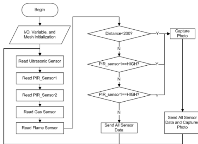
Figure 2 Flowchart Server Mesh
