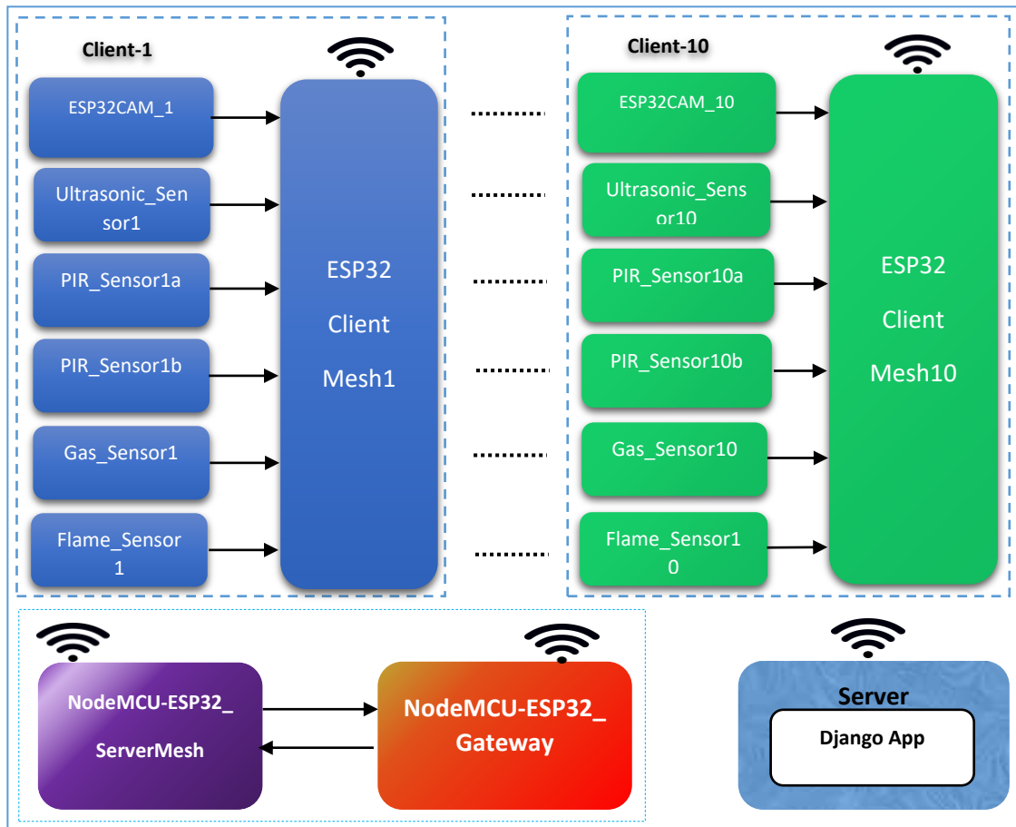
Figure 1 Block Diagram SCHMV1.0
