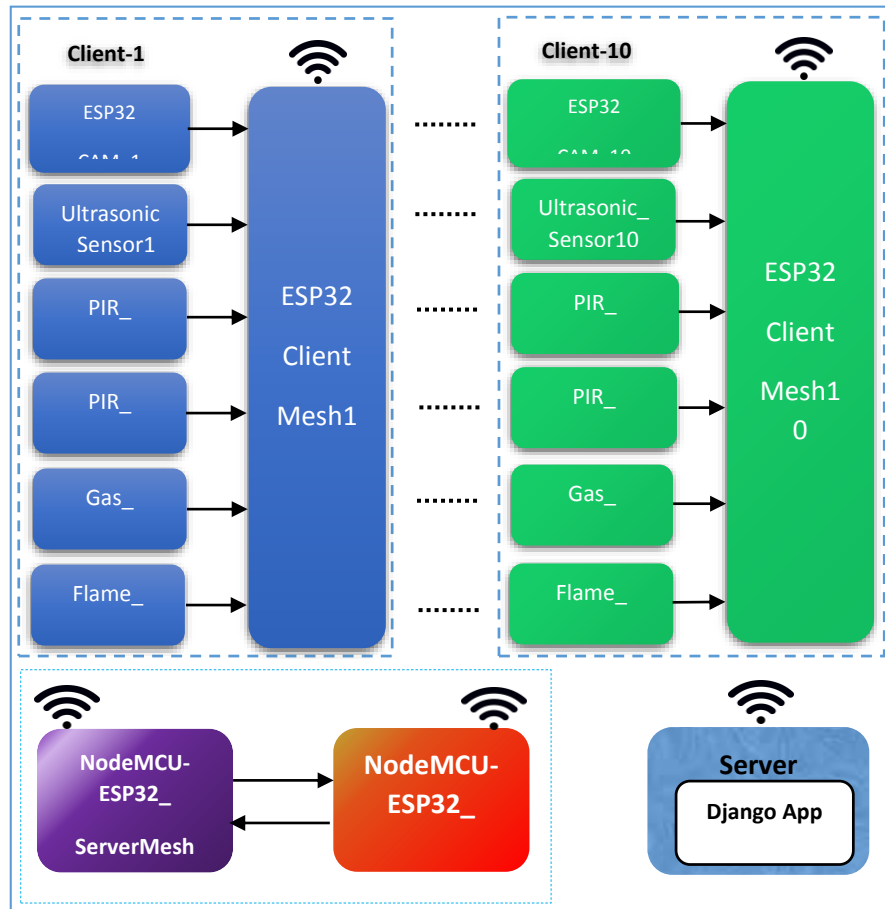
Figure 1 Block Diagram SCHMV1.0
