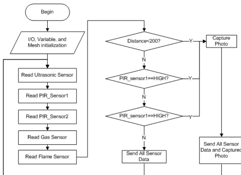
Figure 2 Flowchart Server Mesh
