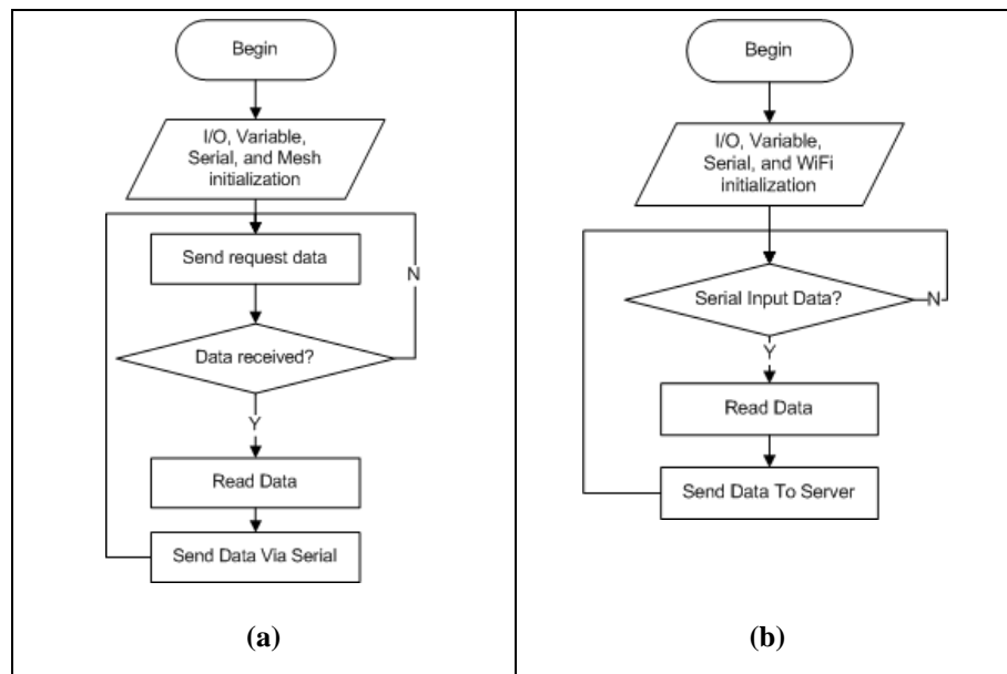
Figure 3 Flowchart (a) Server Mesh and (b) Gateway
