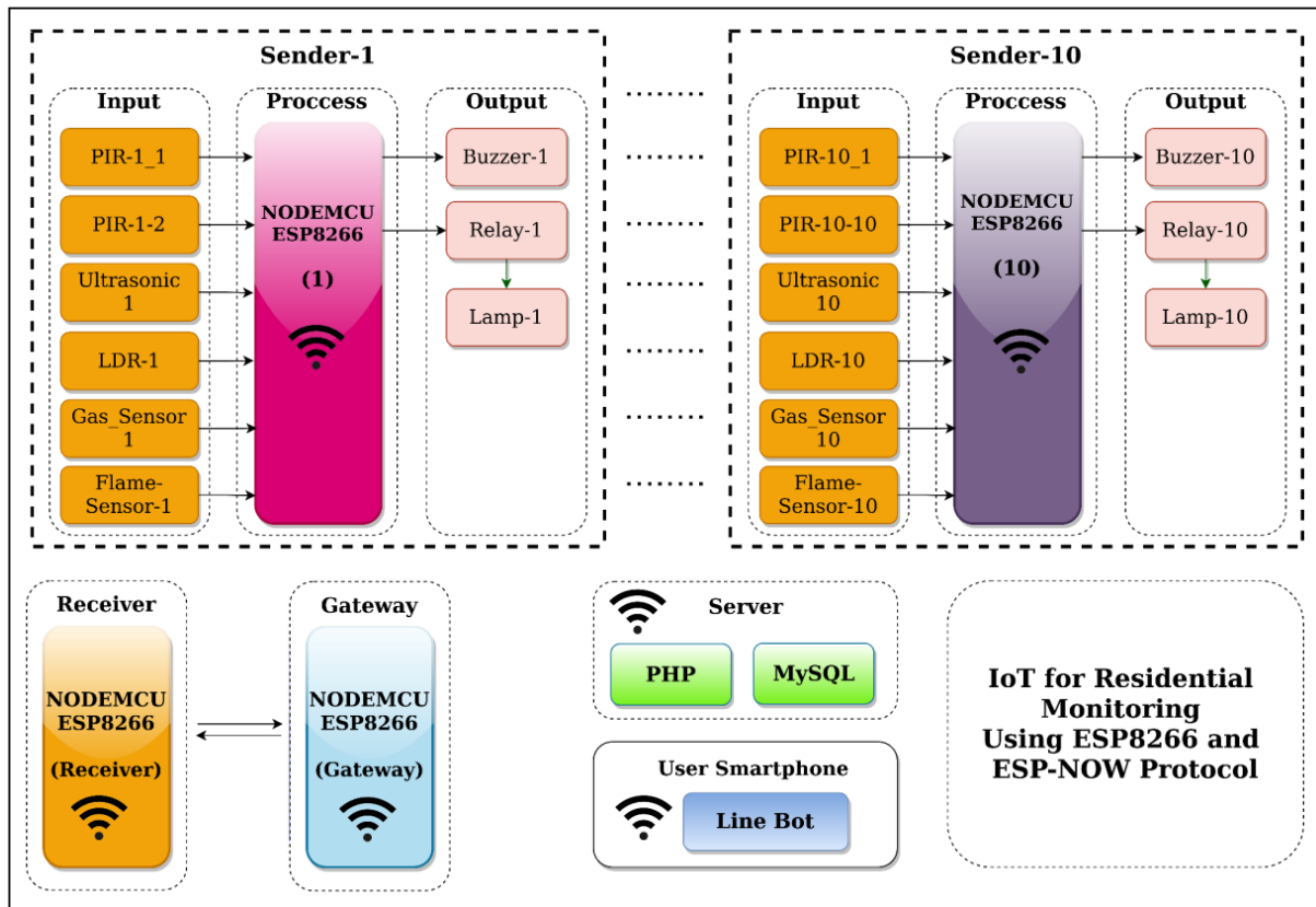
Fig. 2. IoT and ESP-NOW House Monitoring Block Diagram
