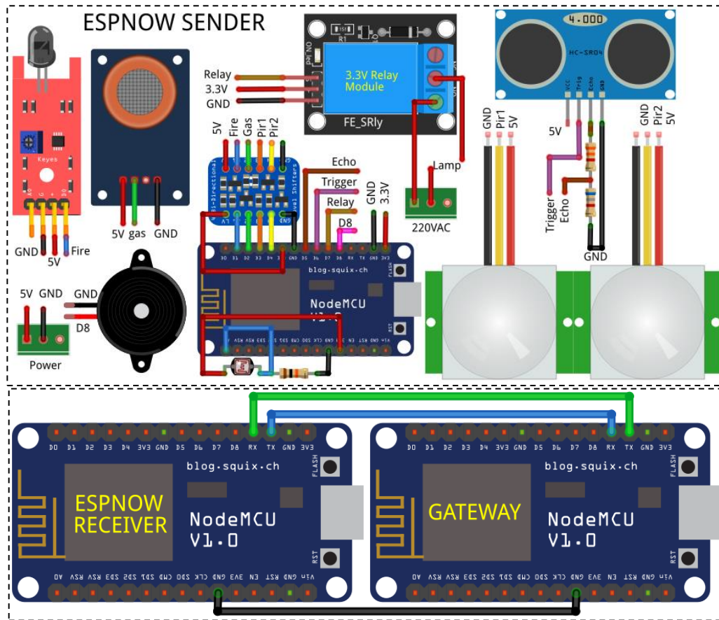
Fig. 3. IoT and ESP-NOW House Monitoring Electronic Design
