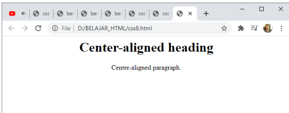
Gambar 8.8. Class Selector
