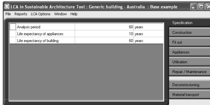
Figure 4. LISA Interface [2]
