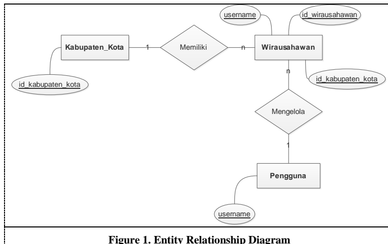
Figure 1. Entity Relationship Diagram
