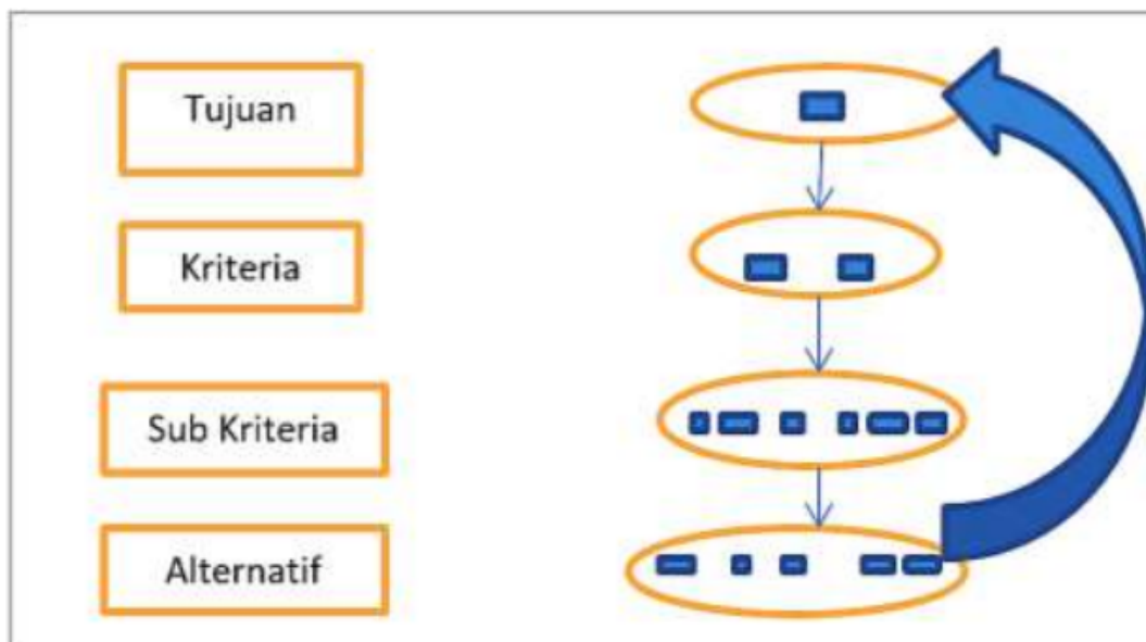
Gambar 7.3 Holarki
