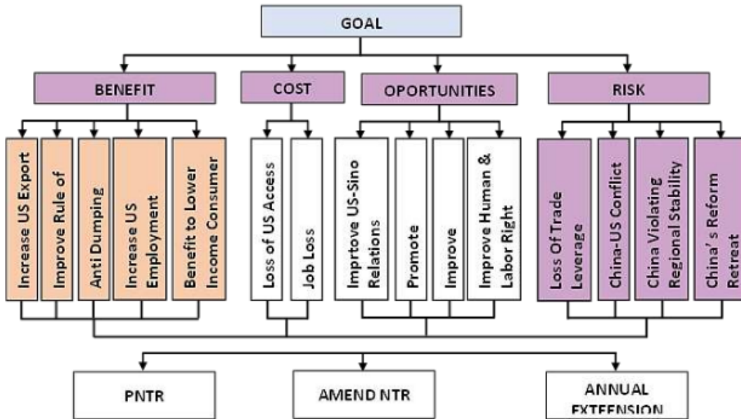
Gambar 7.7 Analisis BCOR
