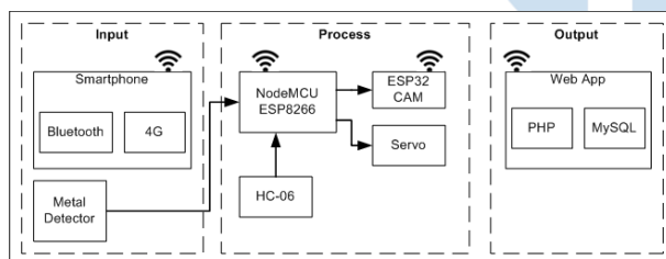
Fig. 1. Portal controller block diagram
