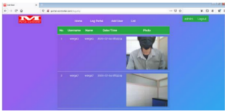
Fig. 10. Log.php page
