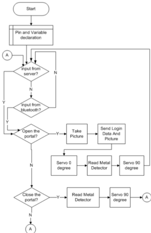
Fig. 2. NodeMCU Portal Controller Flowchart
