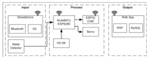
Fig. 1. Portal Controller Block Diagram
