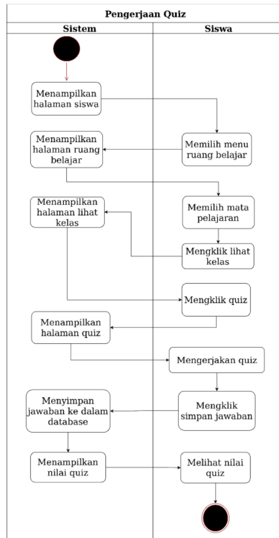
Gambar 4. Activity diagram pengerjaan quiz online
