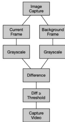
Gambar 2. Cara Kerja Metode Background Substraction
