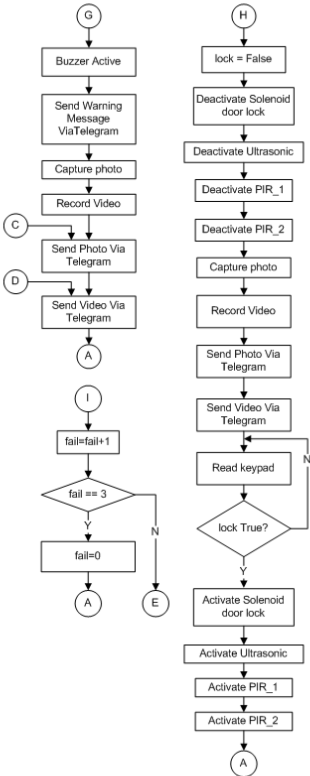
Fig. 3 Flowchart system (continue)
