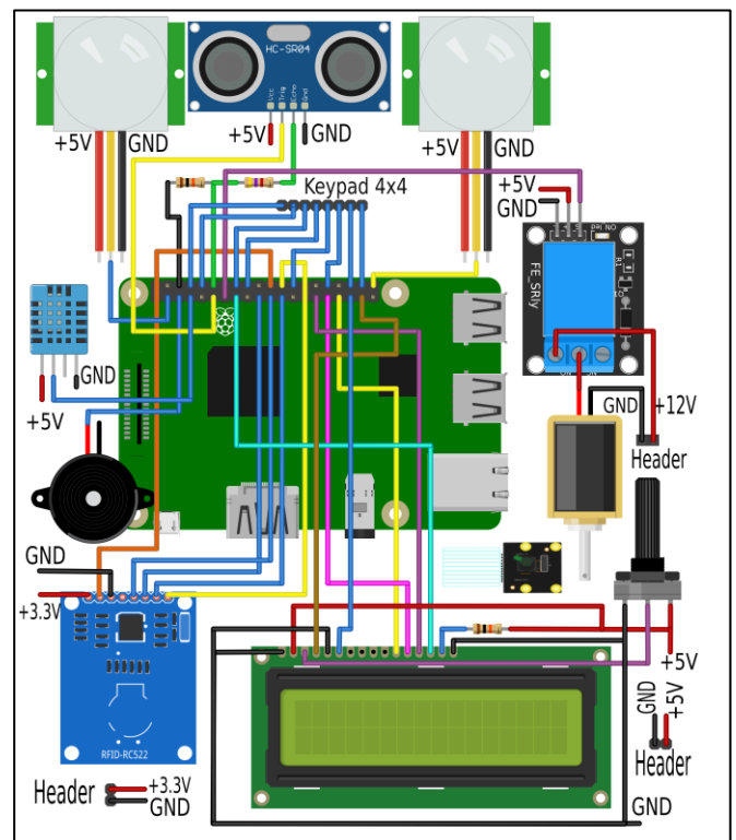
Fig. 3 The electronic circuit of IoT Implementation for Server Room Security Monitoring Using Telegram API
