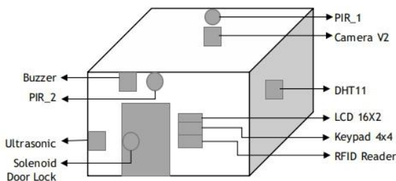
Fig. 2 Design of component placement in the server room
