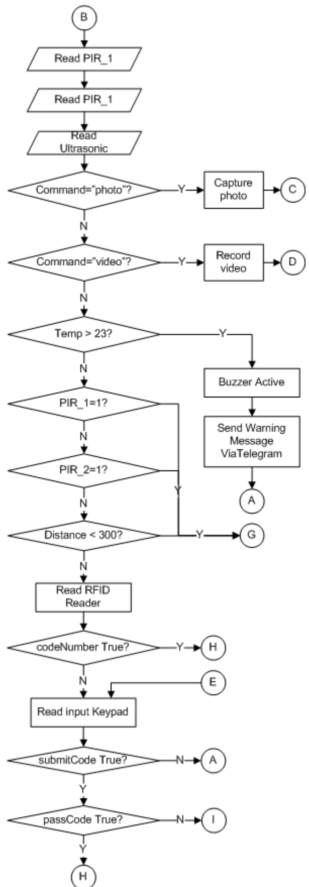
Fig. 3 Flowchart system (continue)
