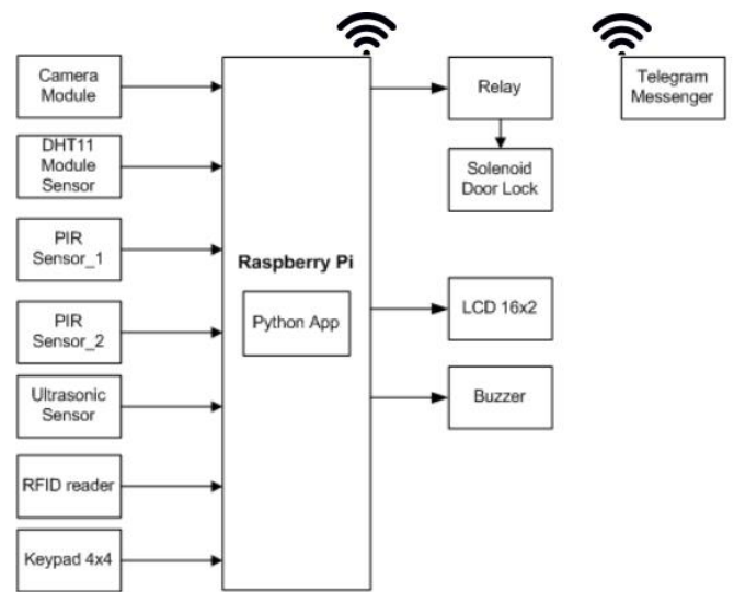
Fig. 1 System Block Diagram IoT Implementation for Server Room Security Monitoring Using Telegram API
