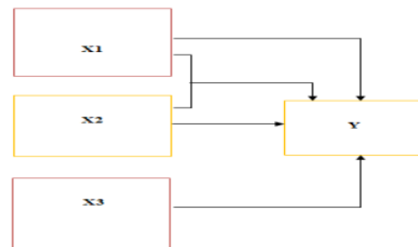
Gambar. 1 Model Hipotesis
