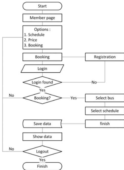
Fig. 2. Flow Chart Online Ticket Booking
