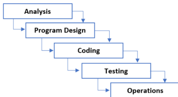
Fig. 1. Waterfall Method
