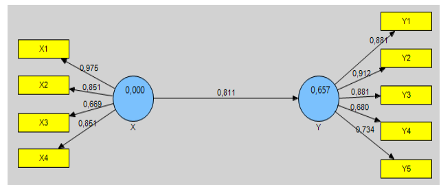
Fig.1 Coefficient Values of Measurement and Structural Models
