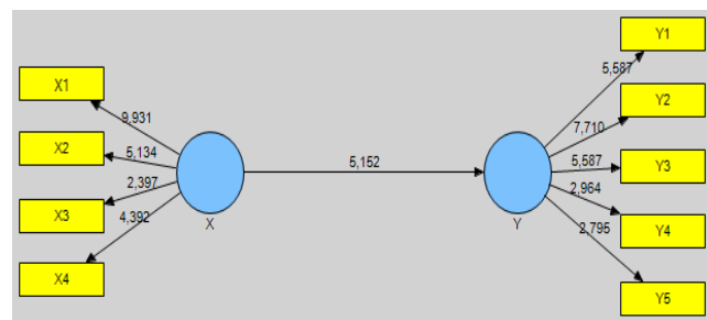
Fig 2. Statistics Values of t-Counted
