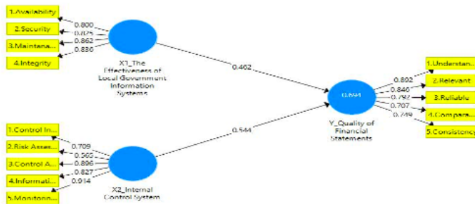
Figure 2. Path diagram of the Partial Least Square (PLS) SEM model approach.
