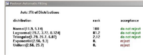
Fig. 8: Auto fit distribution
