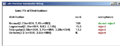
Fig. 6: Distribution stat: Fit
