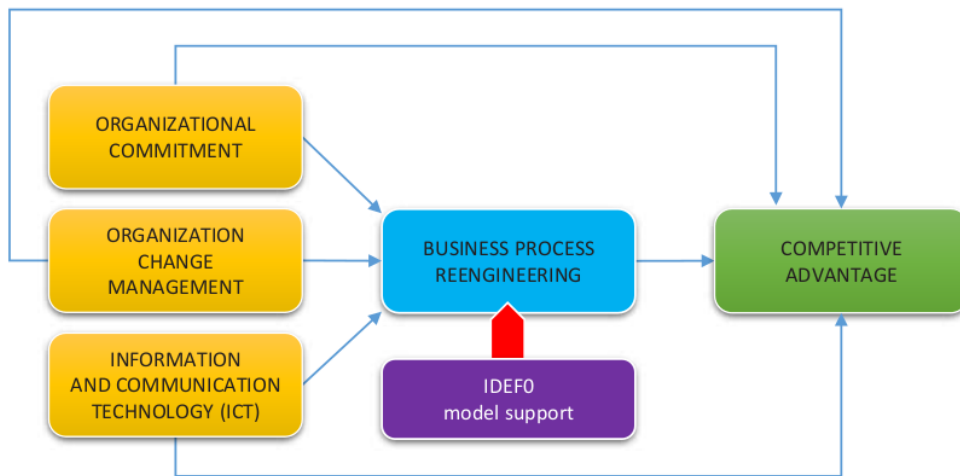
Figure 10. Paradigm model
