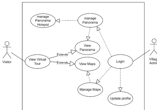
Fig 12. Use Case Diagram of Tourism Village Virtual Tour
