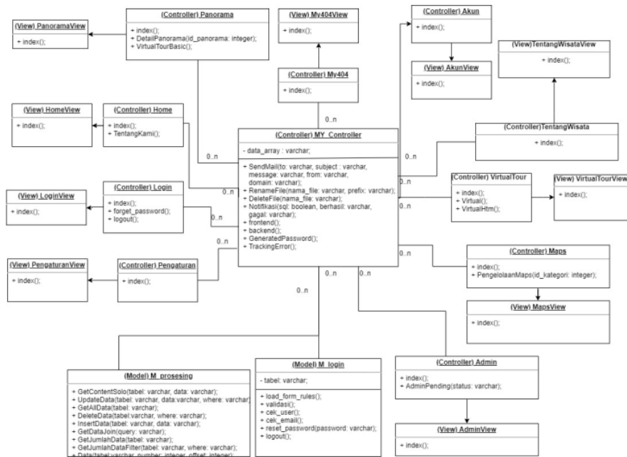
Fig 13. Class Diagrams of Tourism Village Virtual Tour
