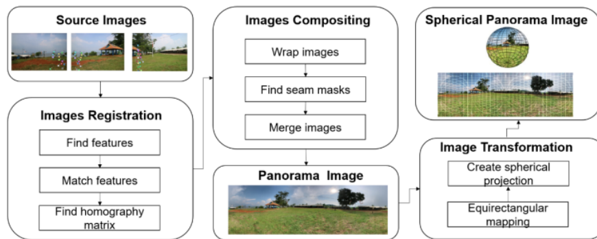
Fig 7. Flowchart of Creating Spherical 360° Panorama Images (Modified)
