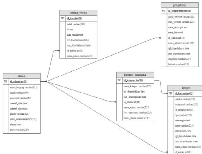
Fig 14. Database Model of Tourism Village Virtual Tour
