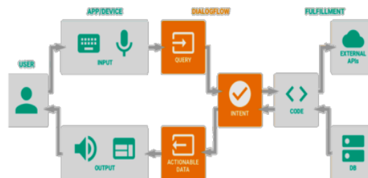
Gambar 2. Model Proses Dialogflow API [12]
