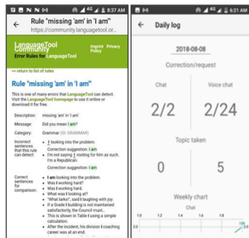
Gambar 15. (a) Antarmuka Grammar Rule, (b) Antarmuka Daily Log
