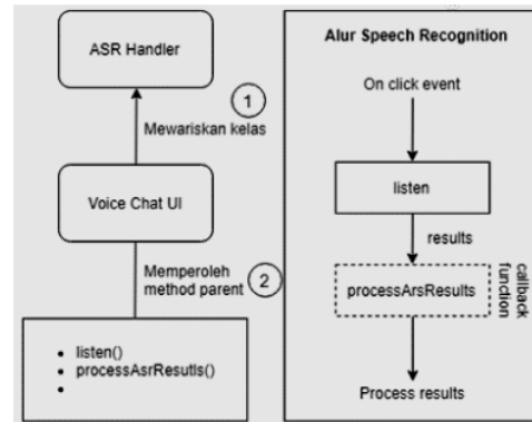
Gambar 7. ASR Handler dan Alur Speech Recognition
