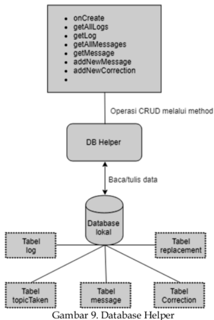
Gambar 9. Database Helper
