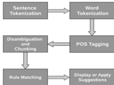
Gambar 3. Model Proses Languagetool API [13]
