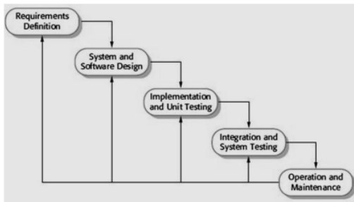
Gambar 1. Model Waterfall
