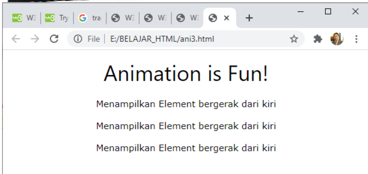
Gambar 12.3. Animate-left
