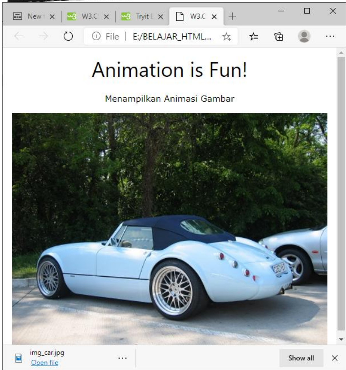
Gambar 12.5. Animate-opacity
