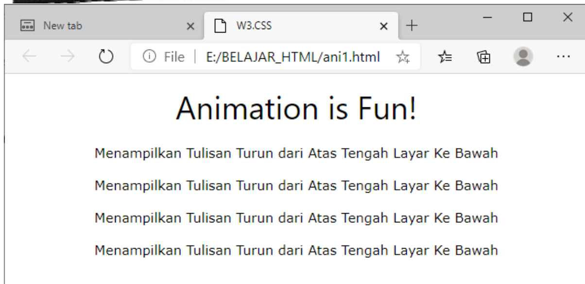
Gambar 12.1. Animate-top
