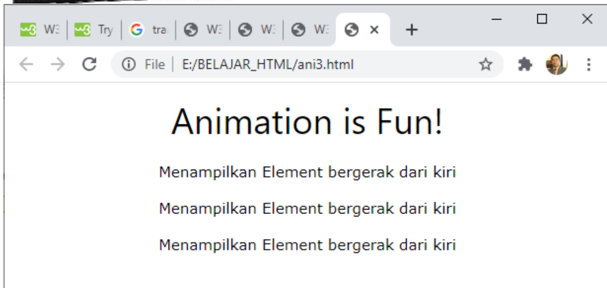
Gambar 12.4. Animate-right
