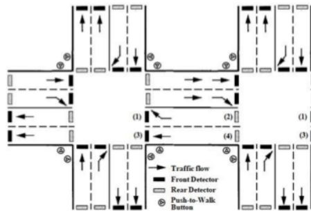
Fig. 1. Example location of the detector and push-to-walk button. (1) Front sensor to detecting a turning vehicle, (2) Rear sensor to detect a turning vehicle, (3) Front sensor to detecting a straight vehicle and (4) Rear sensor to detecting a straight vehicle.
