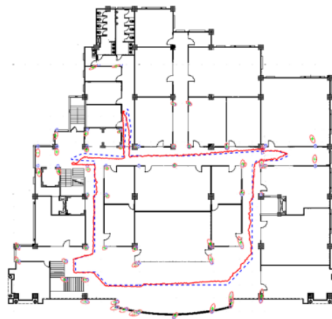
Figure 7. Trajectory prediction from the propose SLAM
