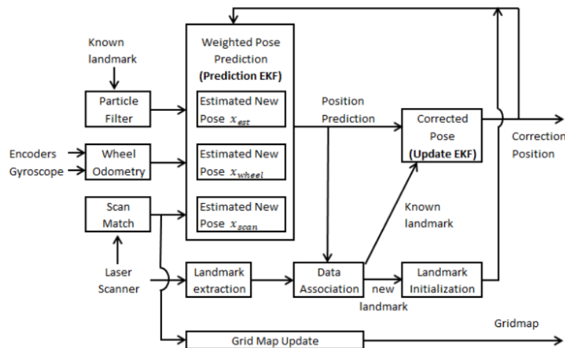
Figure 1. Block diagram of propose SLAM
