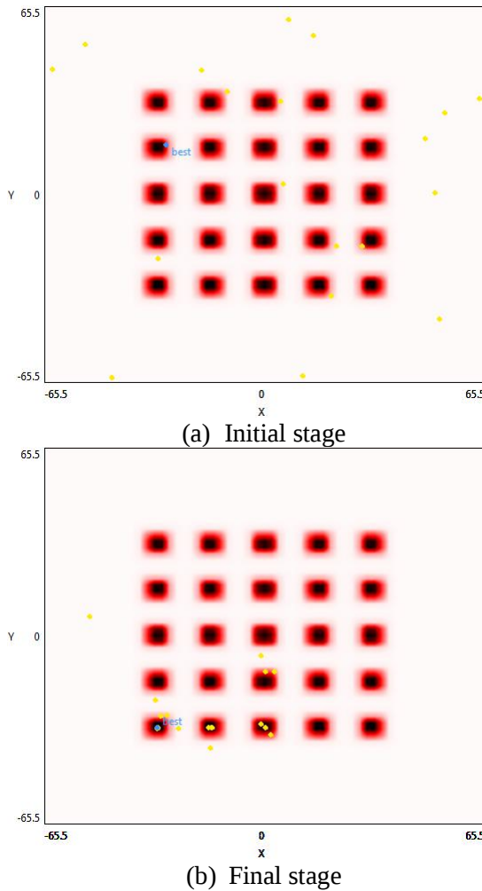
Figure 10. Optimization process for the Shekel's Foxholes Function
