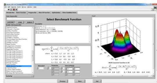
Figure 2. Functions Selection Layers
