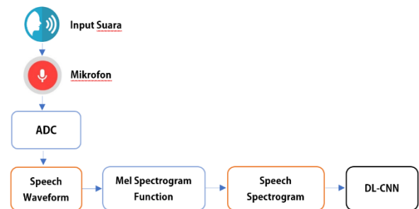
Gambar 3 Diagram blok proses konversi speech waveform ke speech spectrogram
