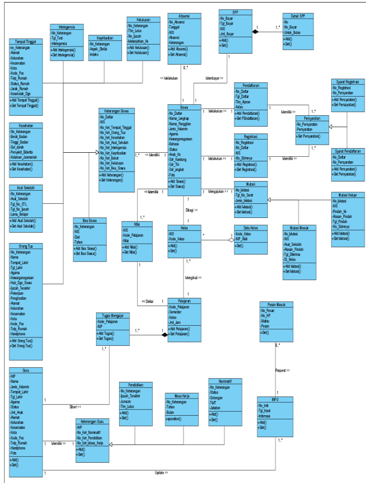
Gambar 4 Class Diagram
