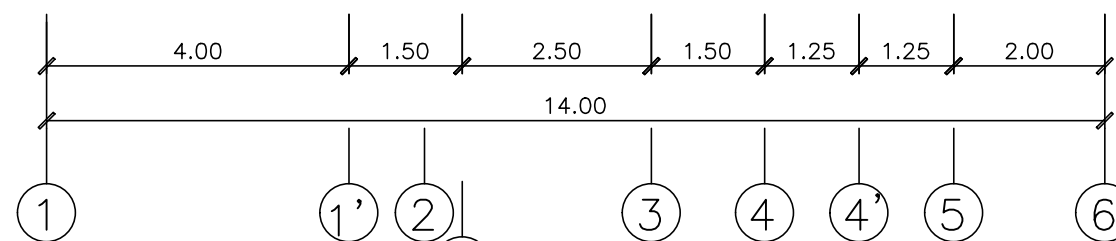
TAMPAK SAMPING KANAN SKALA 1: 100
