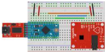
Fig. 9. AD8232 pins connection to Arduino
