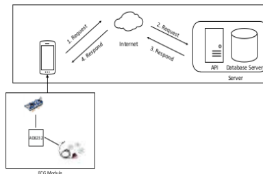
Fig. 7. System Architecture
