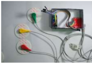
Fig. 12. Tool Implementation
