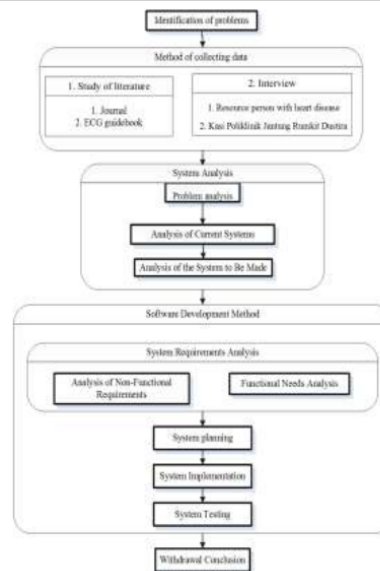
Fig. 6. Research Methodology
