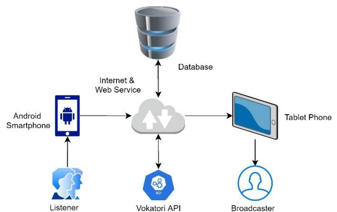
Figure 2. Song title recommendation architecture
