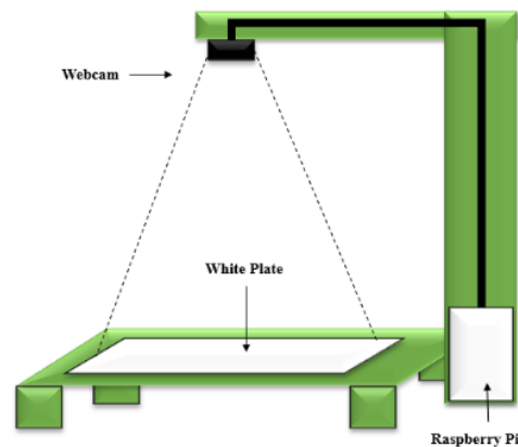
Figure 1. Leaf measuring device design
