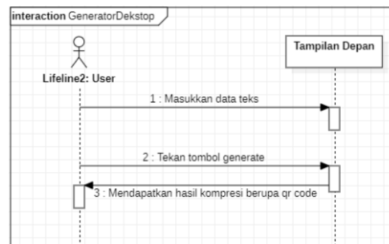
Gambar 5. Sequence diagram aplikasi generator kode QR
