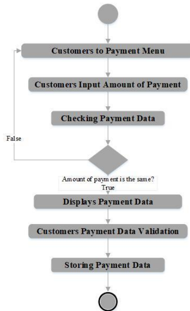
Figure 5. Activity Diagram Payment
