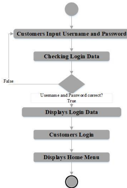
Figure 3. Activity Diagram Login
