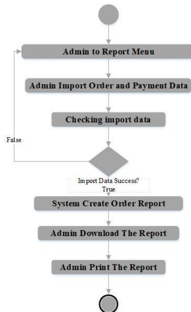
Figure 6. Activity Diagram Order Report
